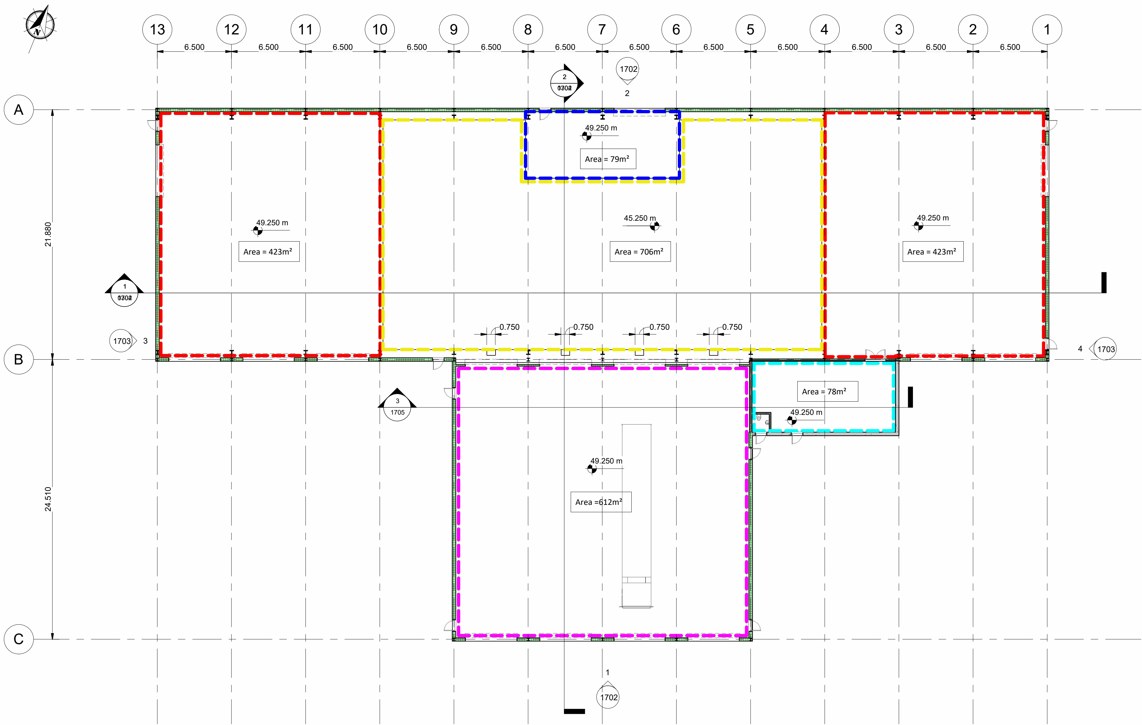
SOLIDS RECEPTION FLOOR PLAN Scale 1 : 200
